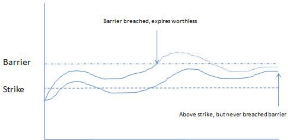
Example "Up and Out", call option
